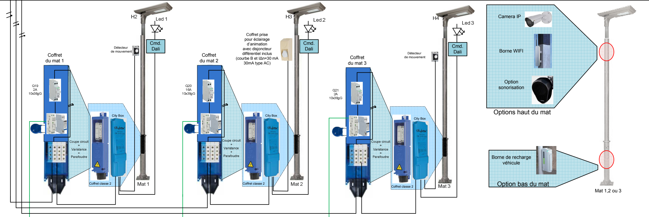
Synoptique Eclairage Type Parking
